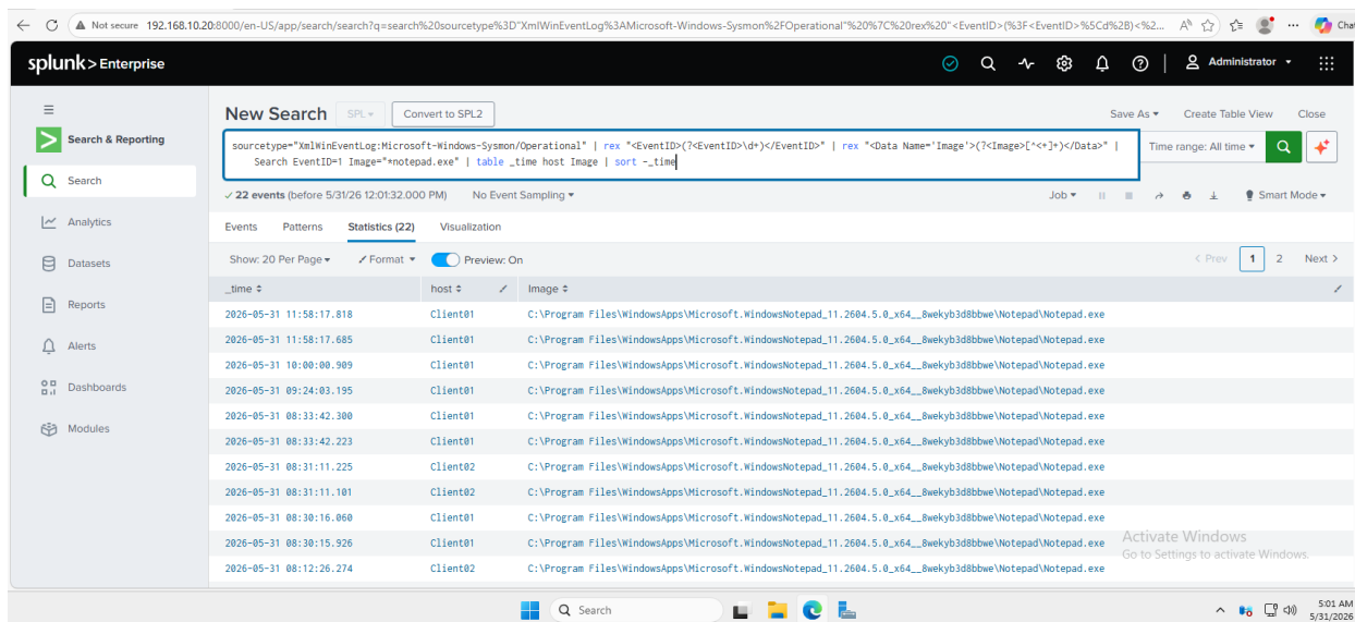
Figure 26 – Sysmon Event ID 1 Detection Results
