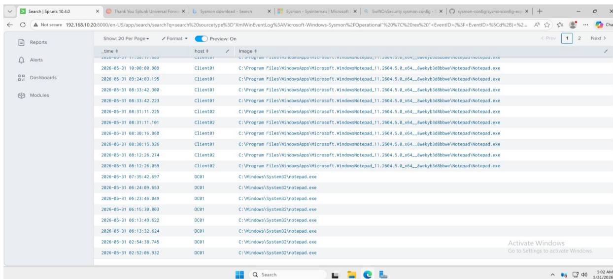
Figure 26 – Sysmon Event ID 1 Detection Results
